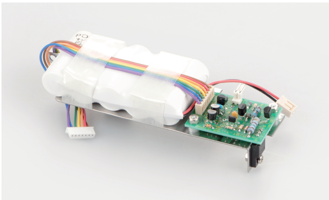
Rechargeable battery pack internal
