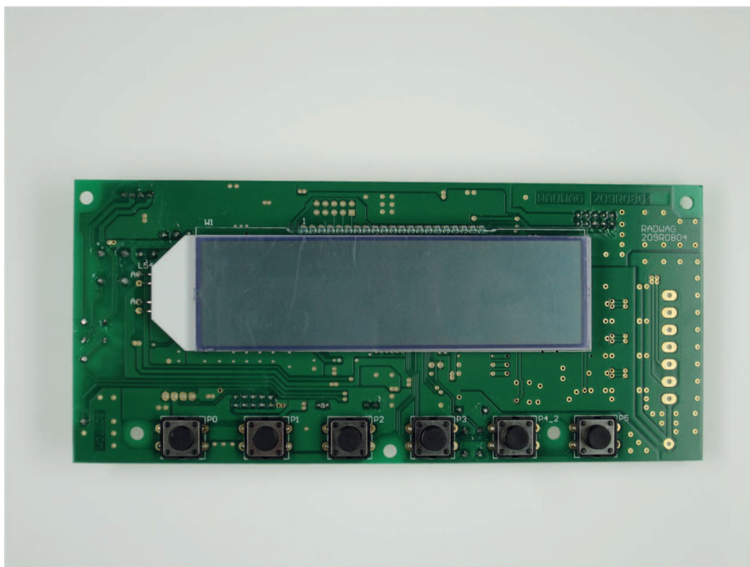
Main PCB, Suitable for model KERN PL-GM
