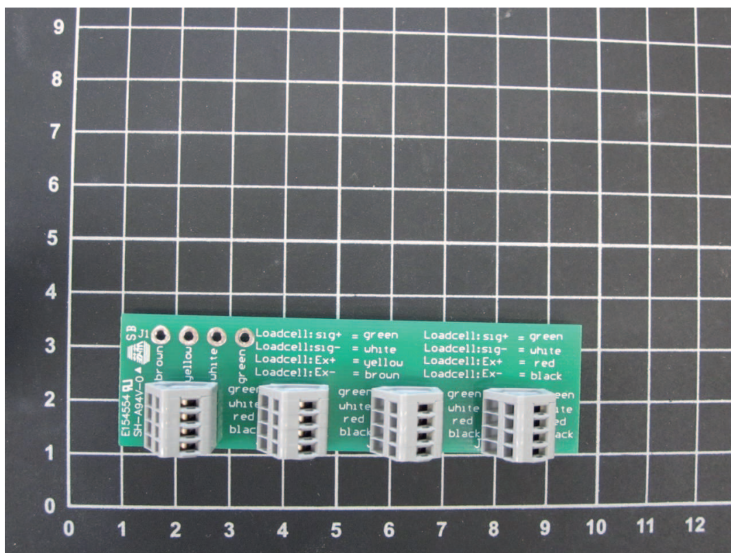
Platine, Junctionbox
