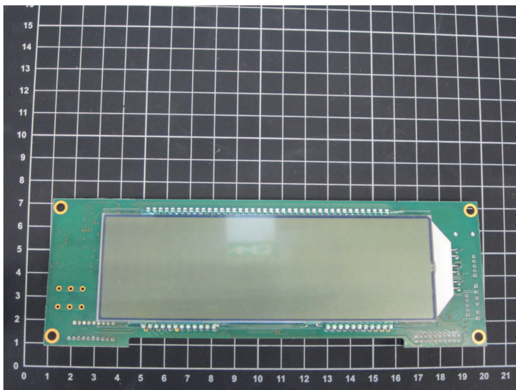
Main PCB, Suitable for model KERN AEJ-C, AEJ-D, AES-C
