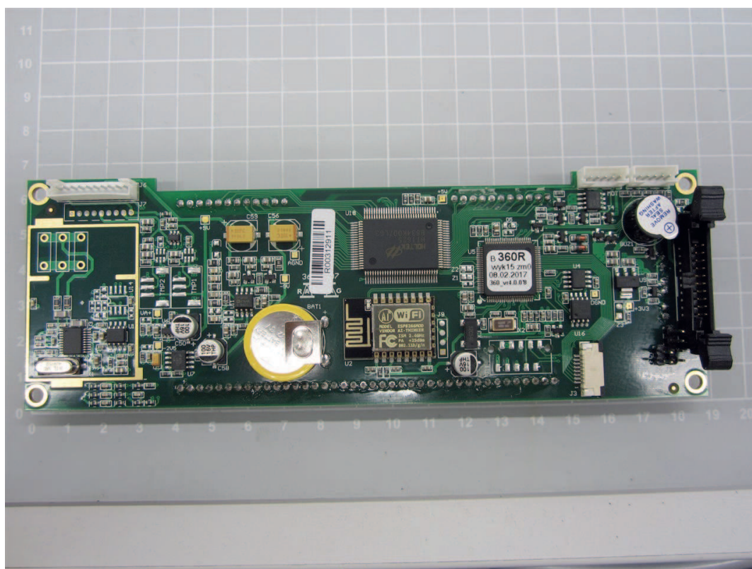
Main PCB RPLJ-C-2003
