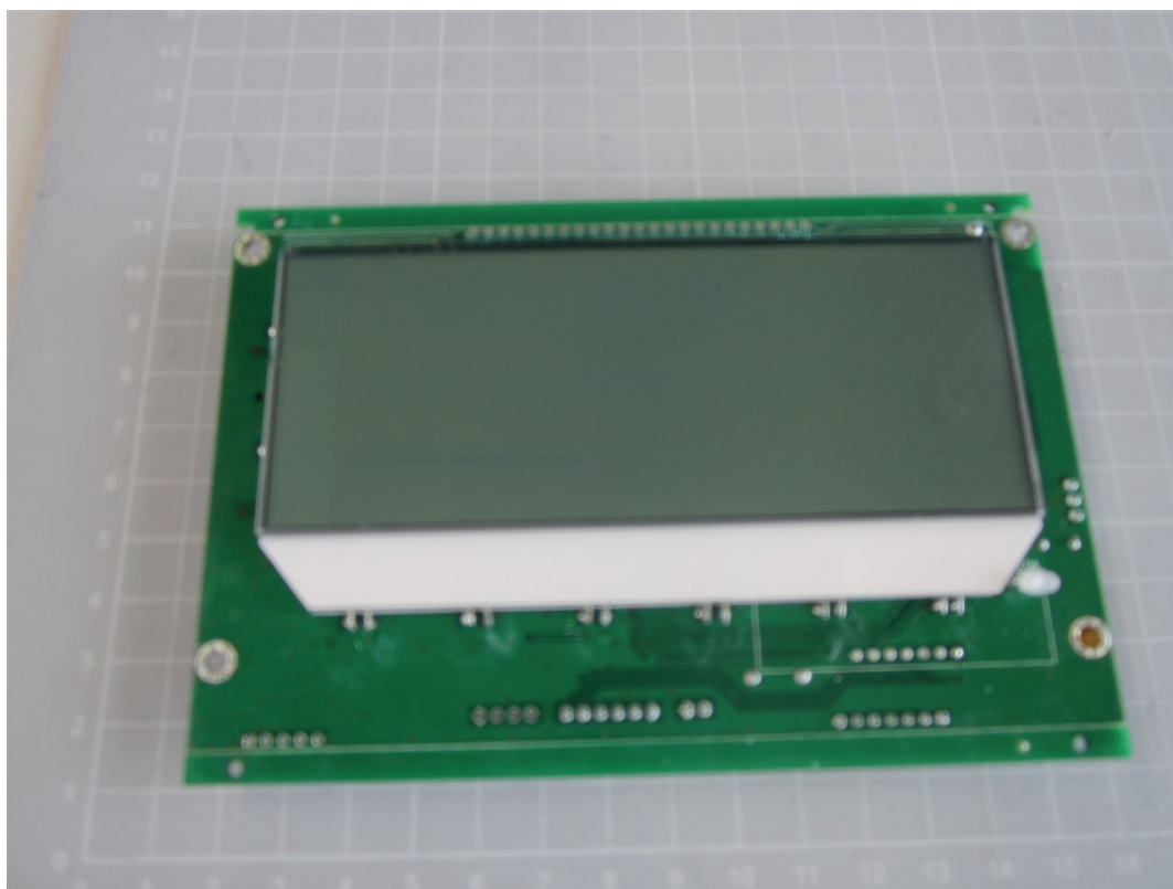
Main PCB, Suitable for model KERN HFD
