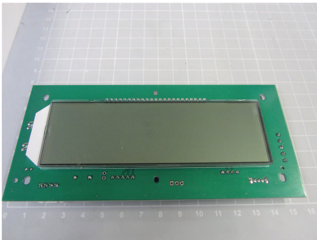
Main PCB, Suitable for model KERN BIC
