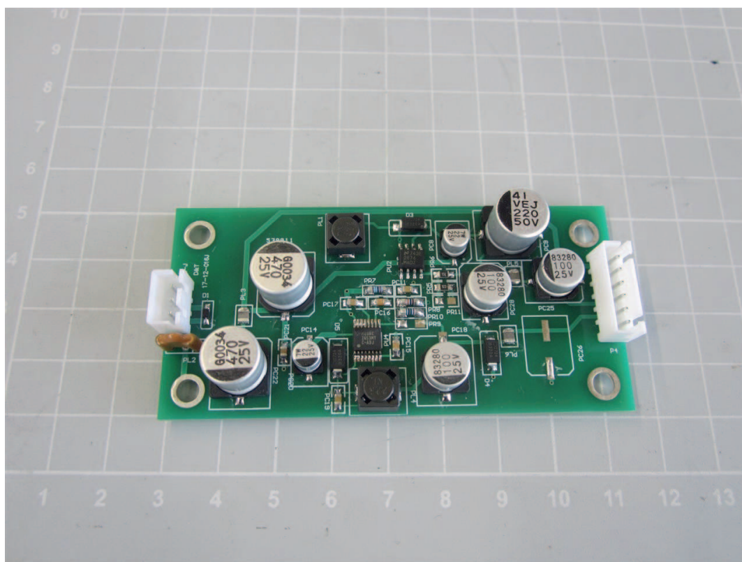
Power supply PCB, Suitable for model KERN ADB 100-4A, ADB 200-4A, ADB 600-C3
