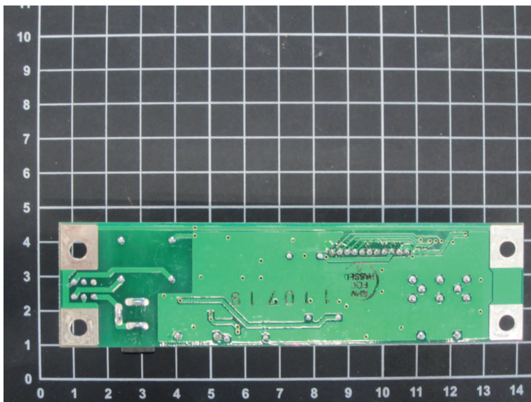
Power supply PCB, Suitable for model KERN ACS/ACJ, ABS-N/ABJ-NM
