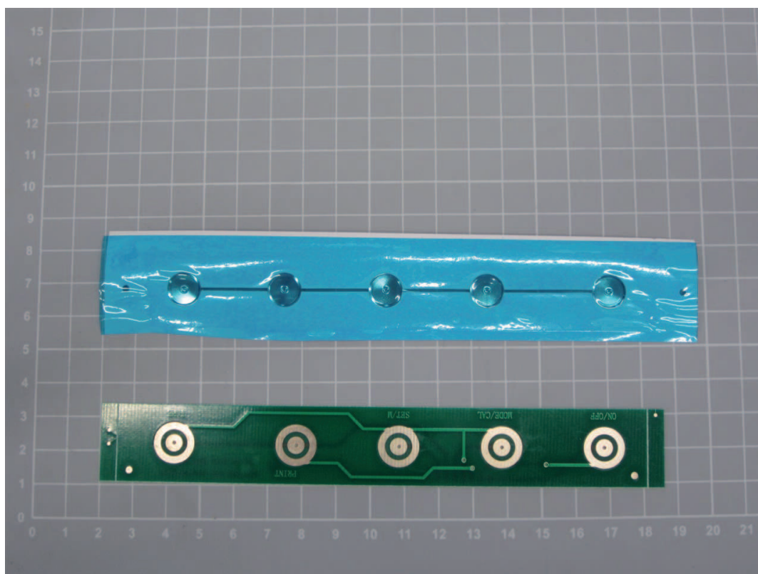
Keyboard PCB, 156x24 mm, Suitable for model KERN DE-D, DE-A
