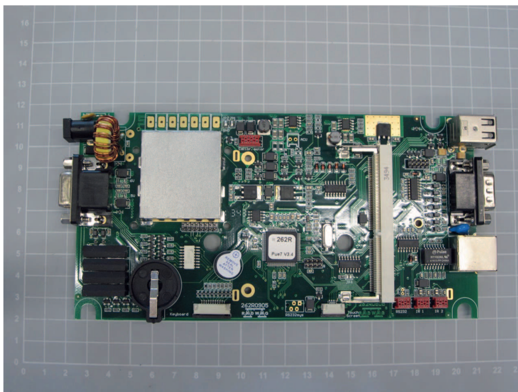
Main PCB, Suitable for model KERN KET-TAM, KET-TM
