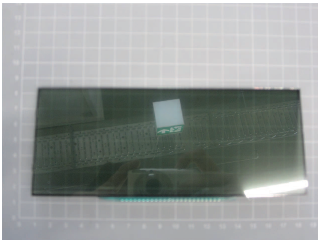
LCD Display, Suitable for model KERN KFB-TM, KFN
