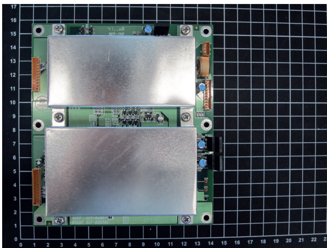
Main PCB, Suitable for model KERN ABT 320-4M
