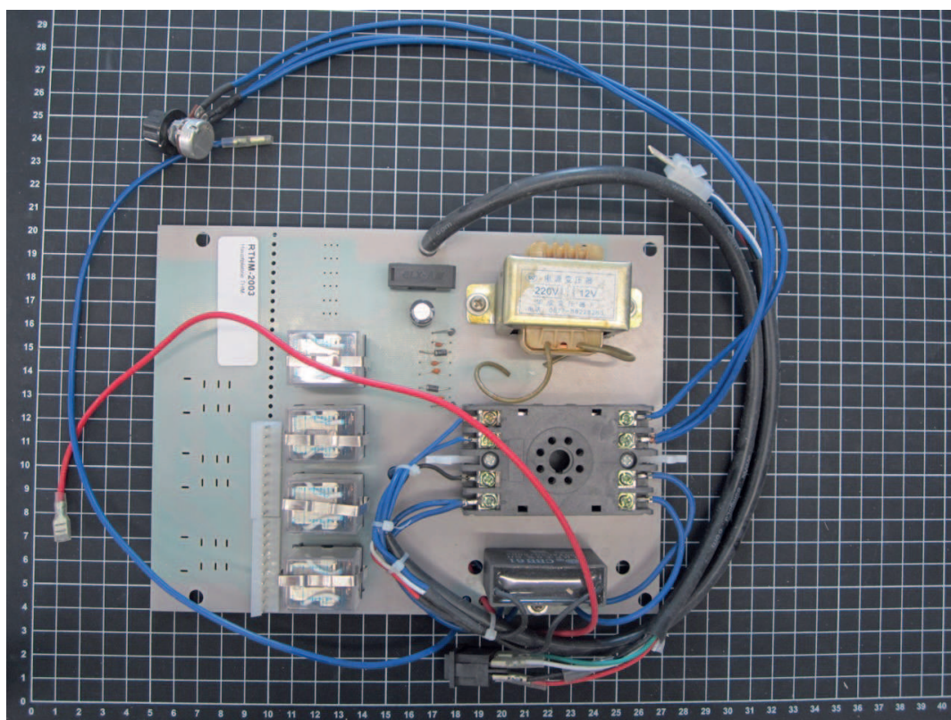
Main PCB RTHM-2003
