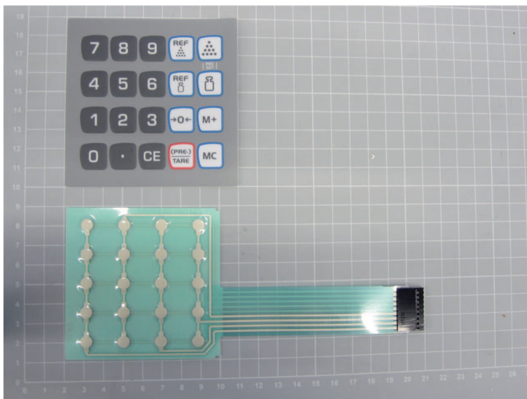
Keyboard overlay, Suitable for model KERN CXB
