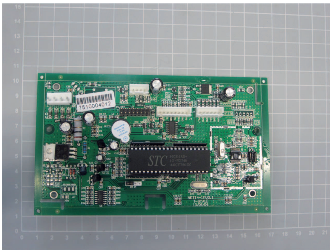
Main PCB, Suitable for model KERN EWJ
