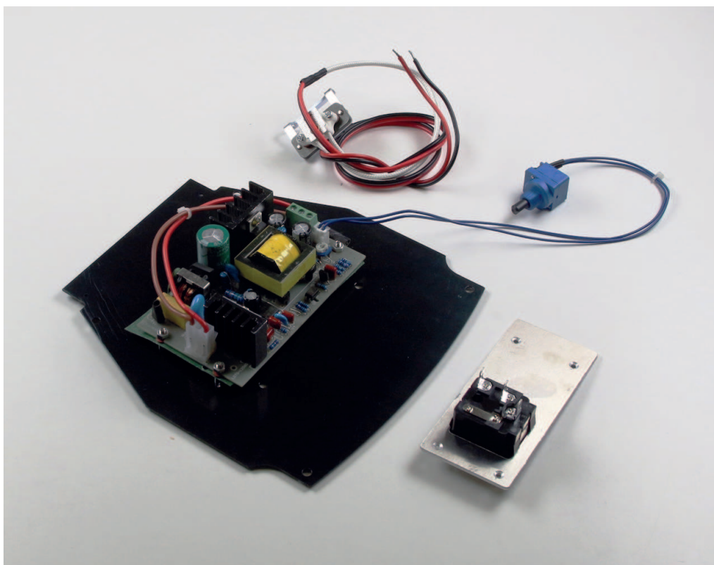
6 V / 30 W Transformer, Suitable for model KERN OCM-1
