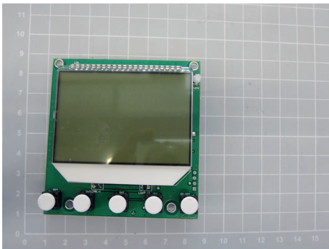
Main PCB, Suitable for model KERN HFA
