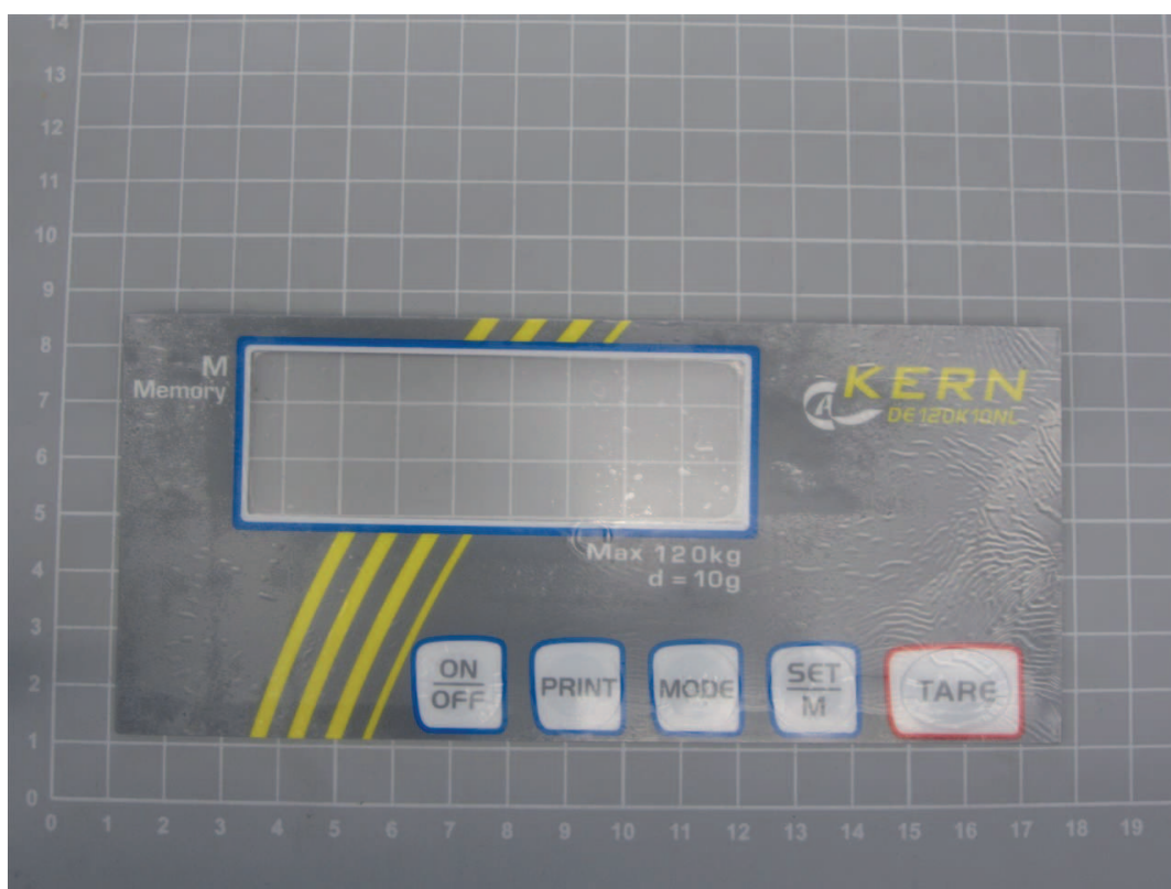
Keyboard overlay, Suitable for model KERN DE 120K10NL
