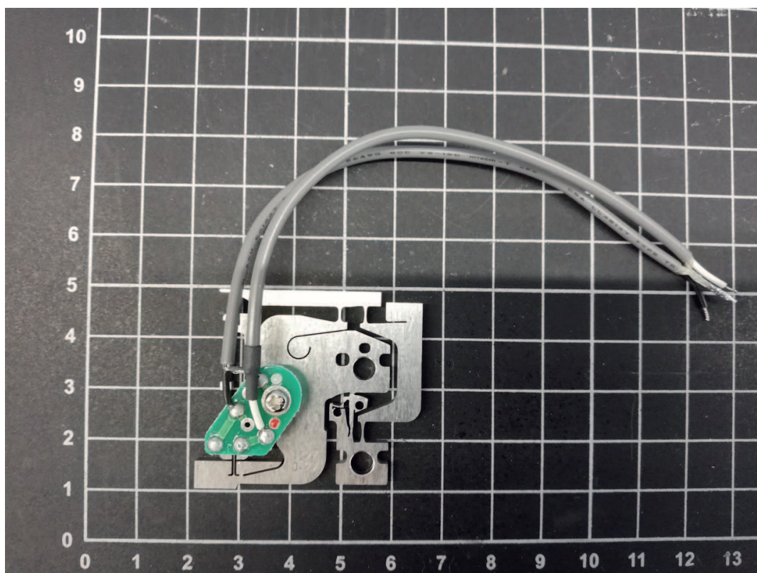
Tuning fork probe
