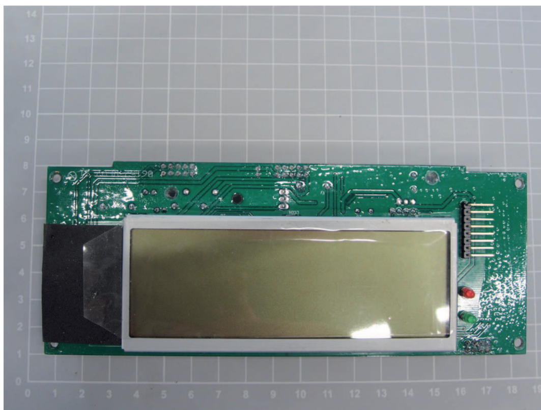
Main PCB, Suitable for model KERN KXE
