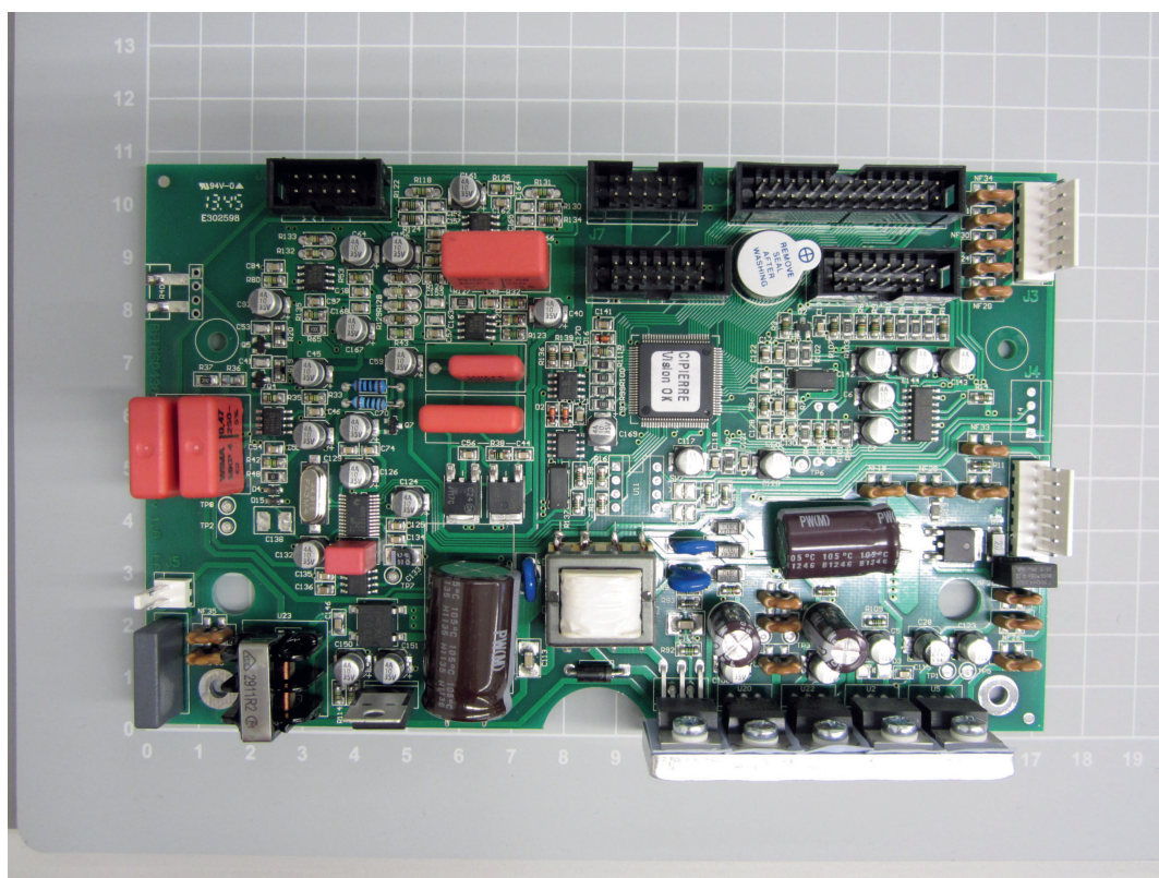
Main PCB, Suitable for model KERN ALS/ALJ-A
